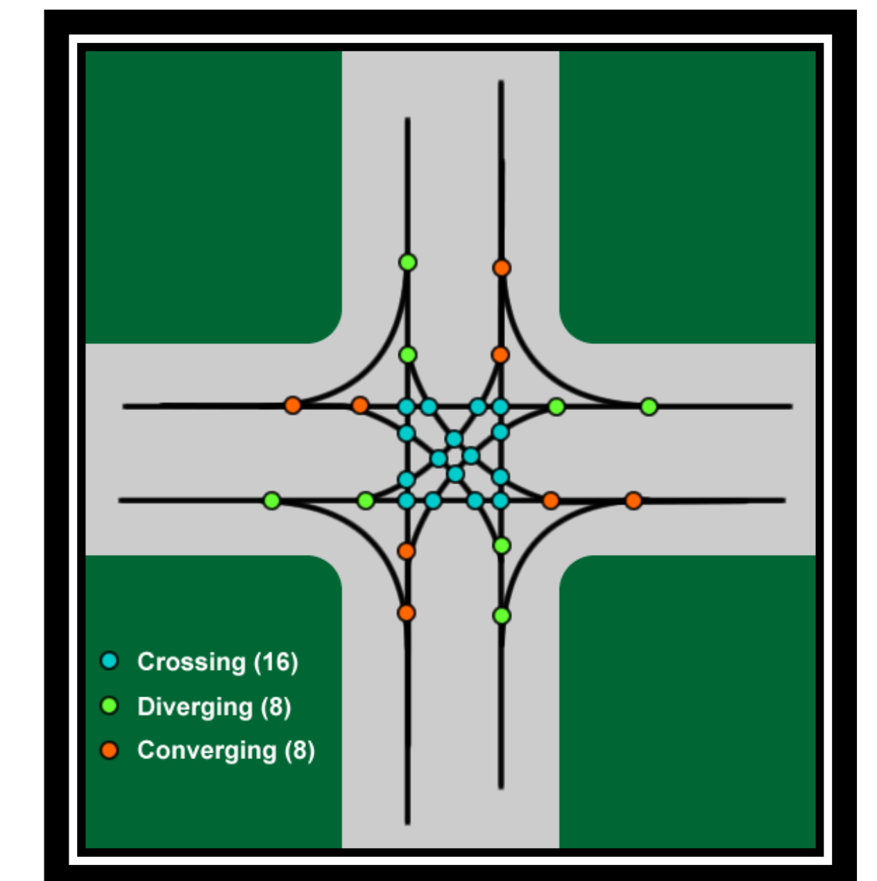
Traditional Intersection
